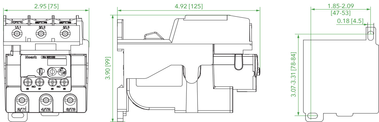
Ex9R100+AD53 Unit: in [mm]
