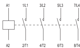
Ex9CS... 4P No Auxiliary
