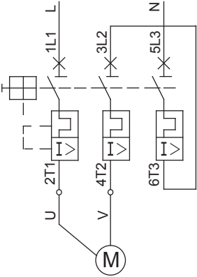
Principle connection diagram of single-phase or DC motor
