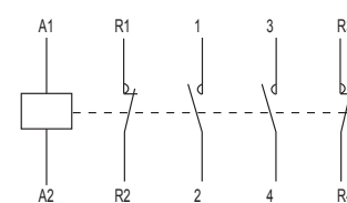
Ex9CMS... 4P 2NO+2NC
