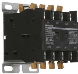
25A, Screw, 50/60Hz, Quad QCT
