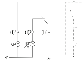
Wiring Diagram of Auxillary Contact
