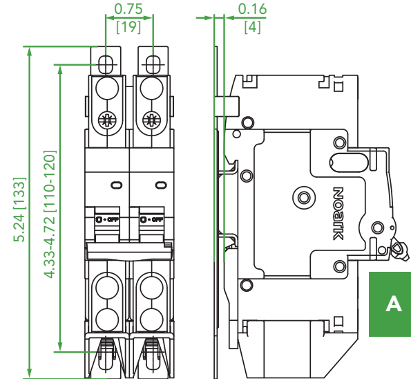
B1NQ Surface Mount Clip 2P Unit: in [mm]
