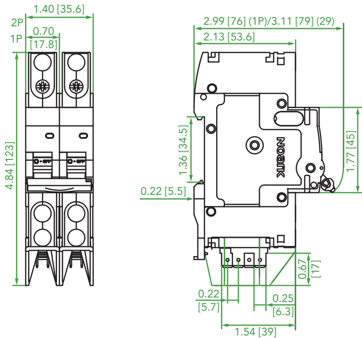
B1NQ with Quick Connection Terminal 1P/2P Unit: in [mm]
